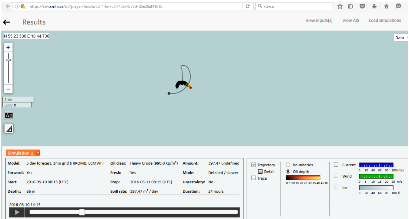
Figure 7. oil leak simulation after 6h 201605101415CET
